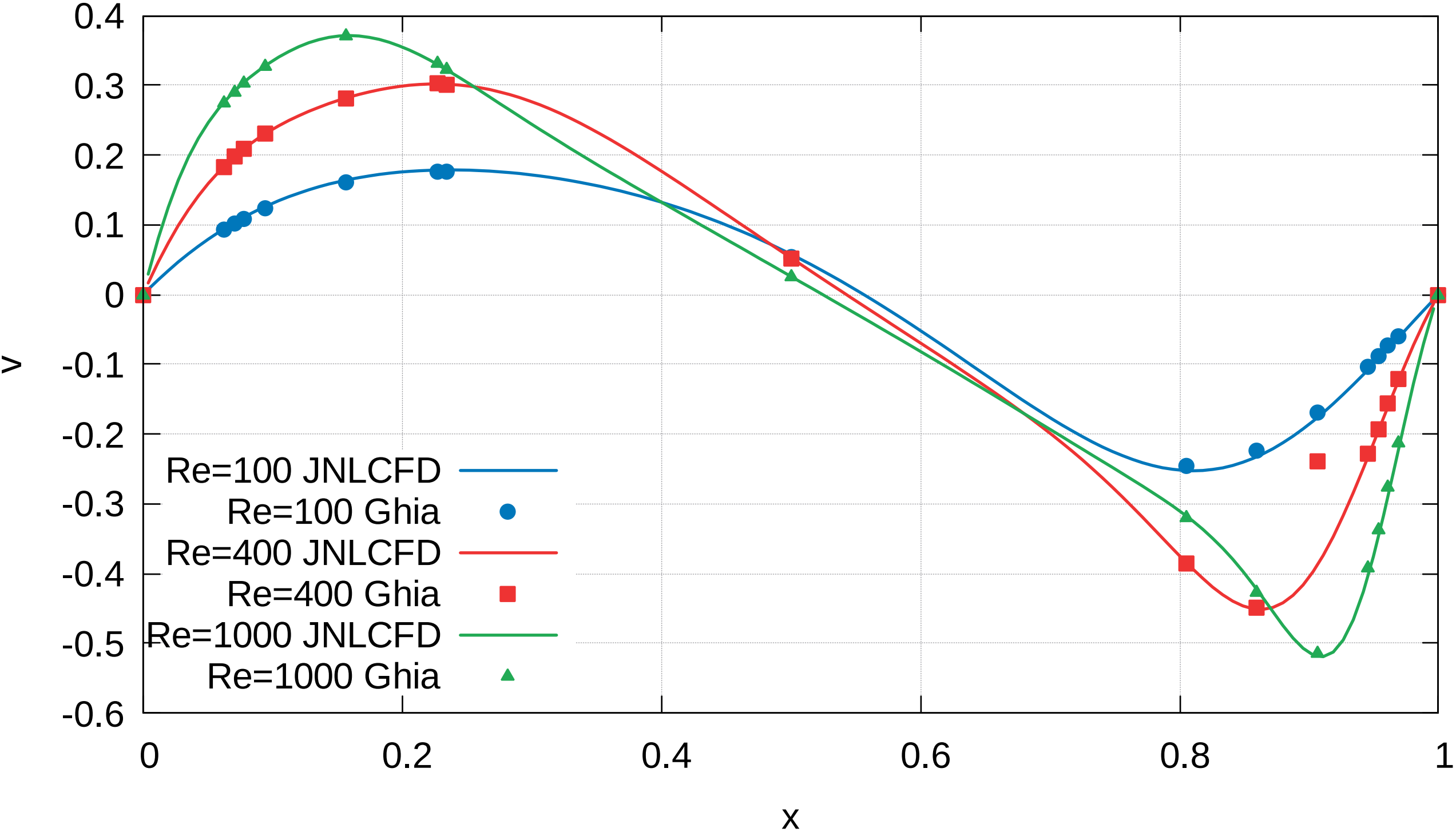
Lid-driven cavity: v at y=0.5 — Ghia et al. validation
