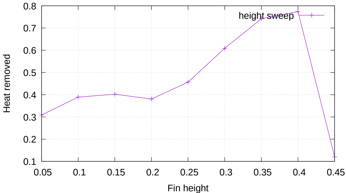
Heat removed vs fin height
