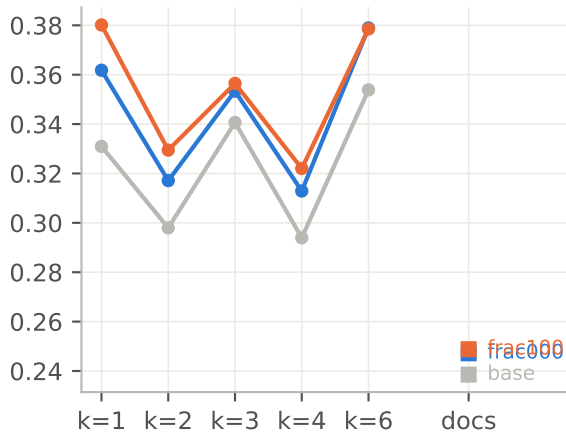
CometKiwi
