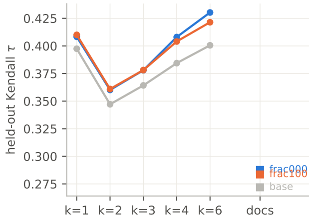
COMET-DA
