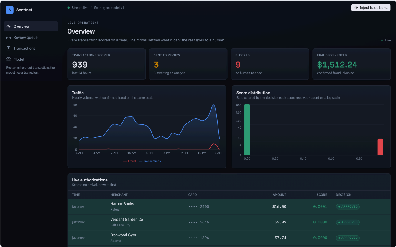
Overview — the live operations dashboard. KPI tiles, an hourly traffic chart with the fraud line pinned near zero (the flat line is the point — fraud is 0.17% of volume), a bimodal score distribution, and a live feed of scored transactions. Say: "every transaction is scored on arrival; the model settles the easy 99%, the rest goes to a human."
