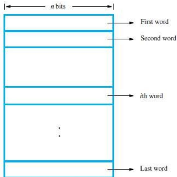
Figure 2.1 Memory words.
