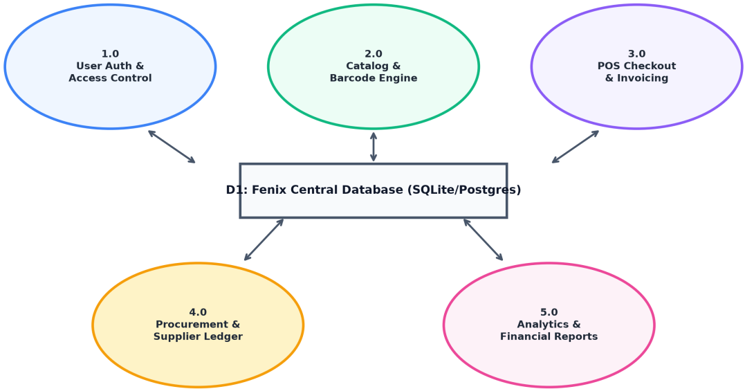
Data Flow Diagram (DFD Level 1 – Core Processes)
