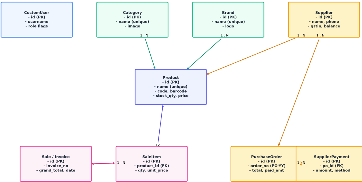
Entity Relationship (ER) Diagram
