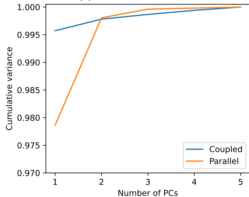
(c) PCA cumulative variance
