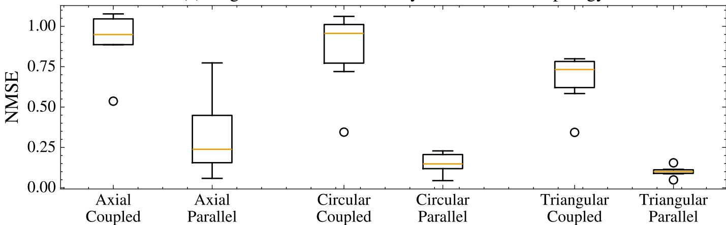
(c) Angle-estimation NMSE by waveform and topology
