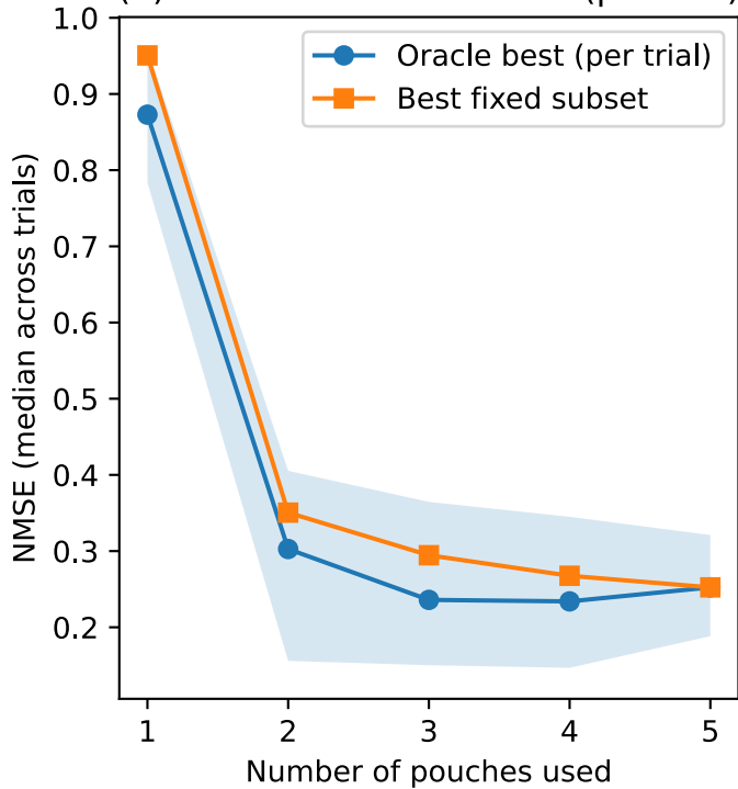
(a) Sensor-count trade-off (parallel)
