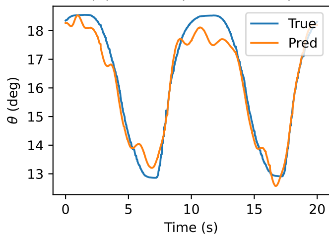
(a) Parallel (Axial 1-5 PSI)
