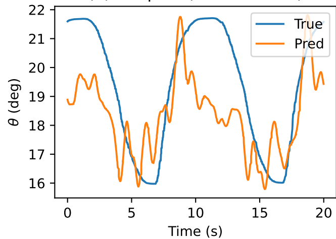
(b) Coupled (Axial 1-5 PSI)
