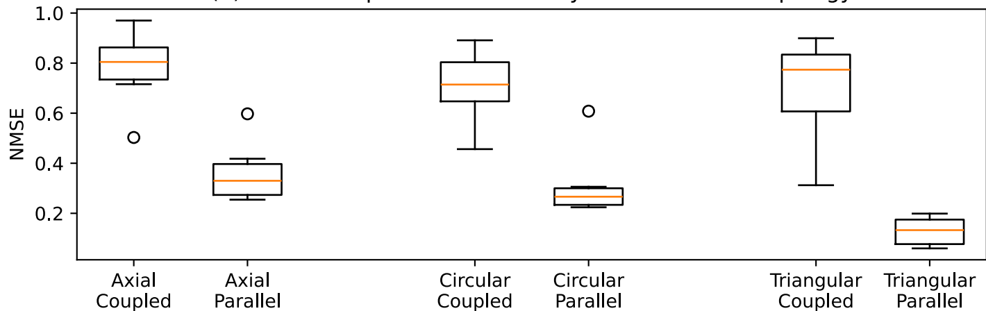
(b) 1 s-ahead prediction NMSE by waveform and topology
