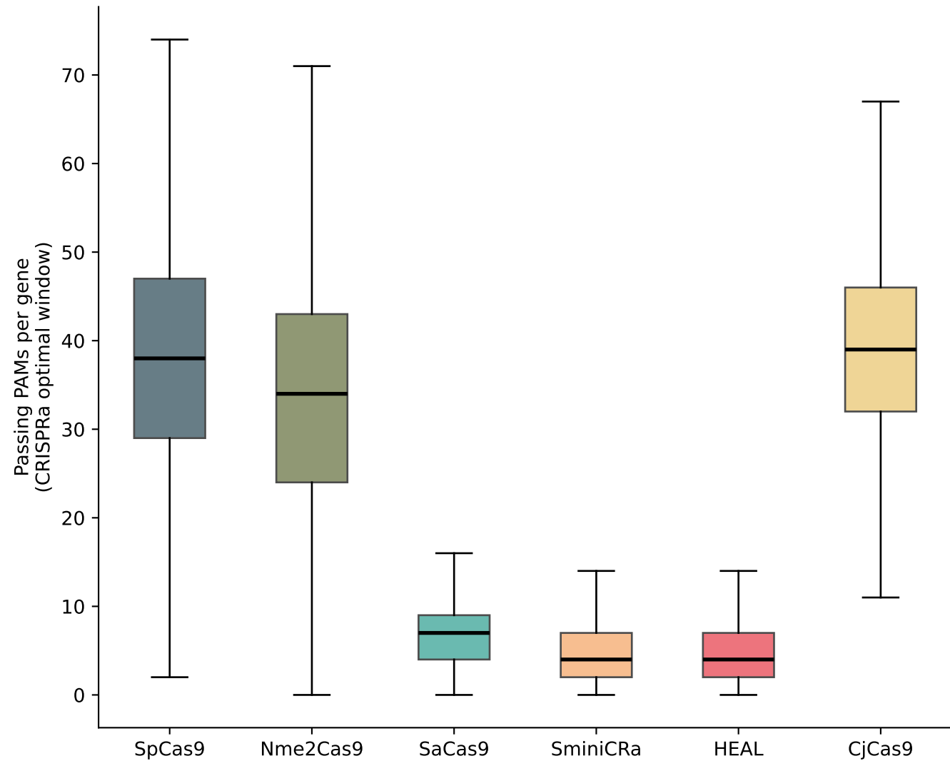
A PAM count distribution (genome-wide)
