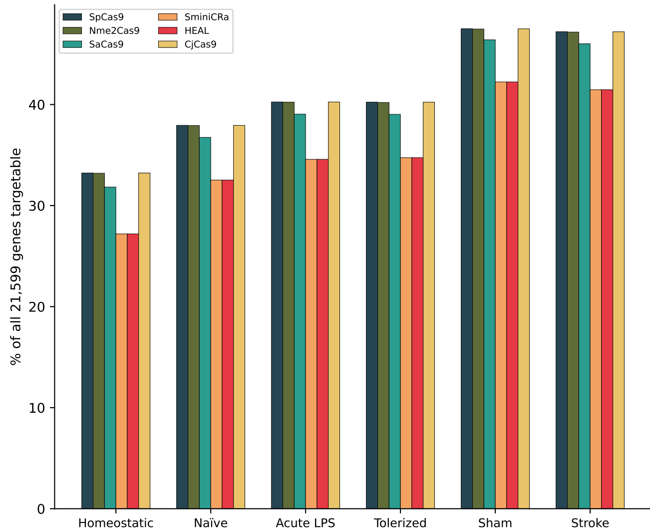
B Genome-wide targetability by state
