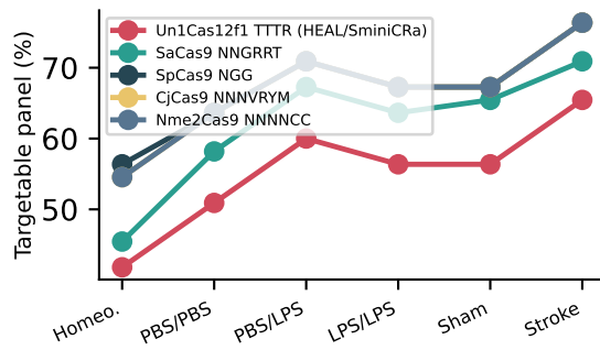
B Five nuclease/PAM classes
