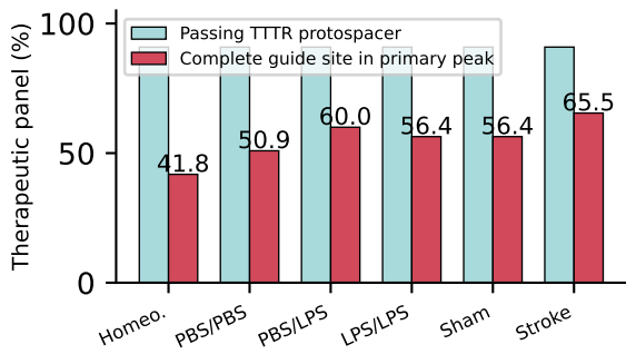
A Sequence versus guide-site support
