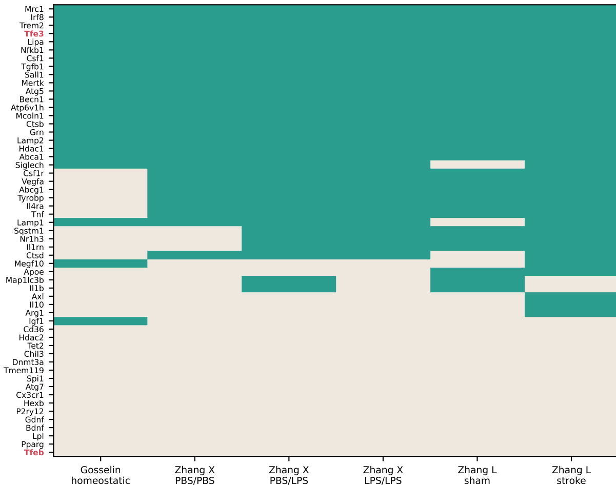
C Guide-specific Un1Cas12f1 support for all 55 locked genes
