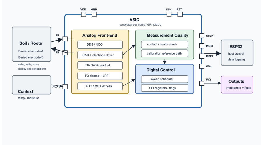
Figure 1: Nopal-Sense ASIC functional architecture
