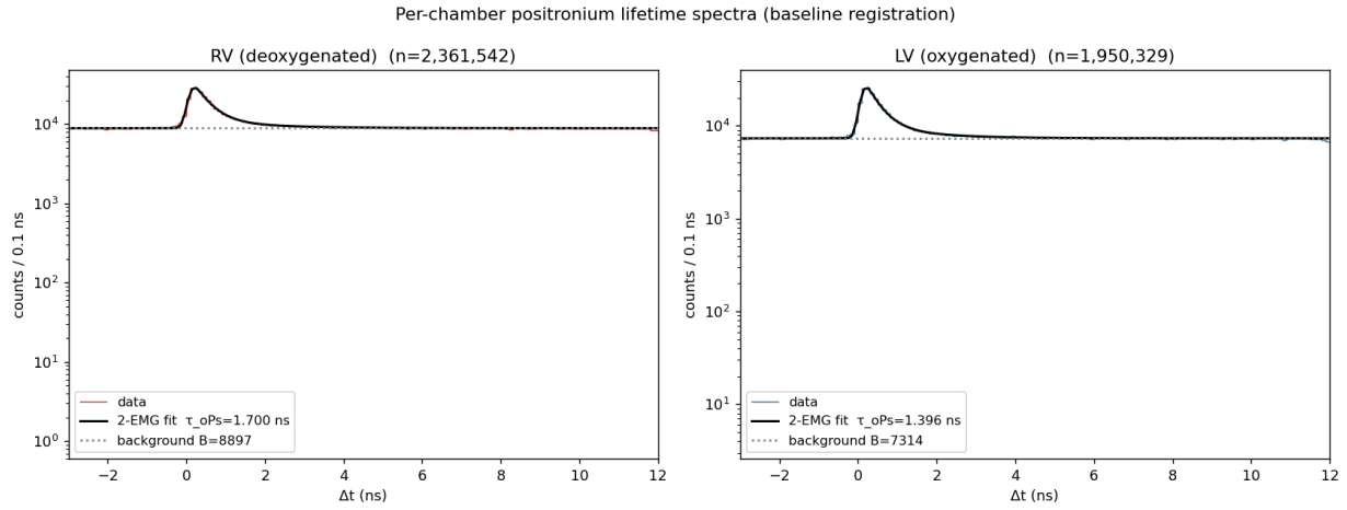
Figure 1. Per-chamber positronium-lifetime spectra ( \Delta t histograms, log scale) for the right and left ventricles at baseline registration, with the background-plus-two-component EMG fits and the fitted flat background. The o-Ps signal is a modest excess over a large accidental background; \tau_{\text{oPs}}(\text{RV}) = 1.700 ns, \tau_{\text{oPs}}(\text{LV}) = 1.396 ns.
