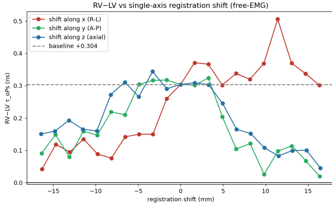
Figure 3. RV-LV lifetime difference versus single-axis registration shift ( \pm 16 mm) along each axis. The difference stays positive across the full tested range.
