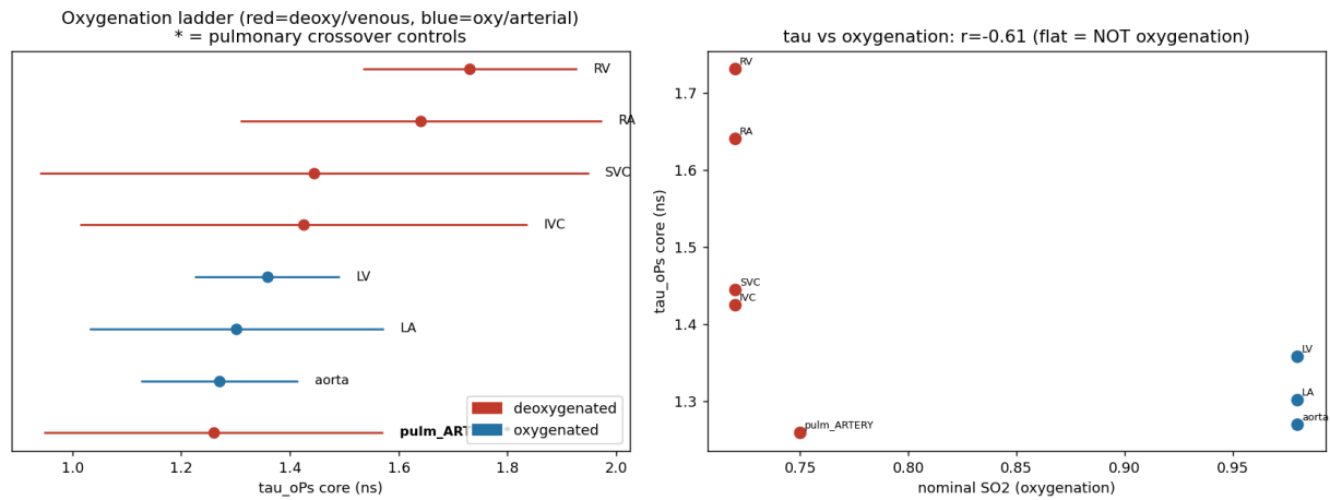
Figure 5. Oxygenation ladder. (Left) per-compartment o-Ps lifetime, coloured by oxygenation class, with the pulmonary crossover controls highlighted; (right) lifetime versus nominal oxygen saturation. The flat trend and the null pulmonary-artery–aorta pair indicate the contrast does not track oxygenation.
