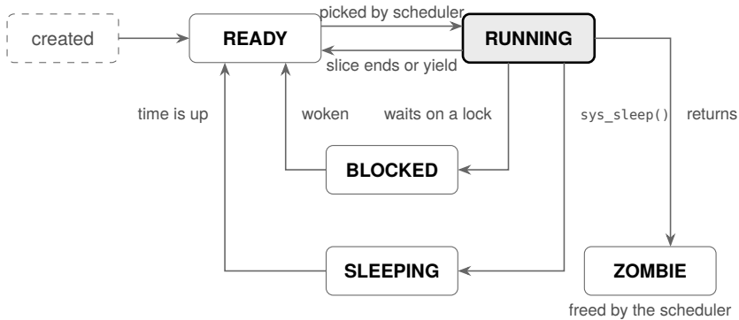
Figure 4.1: Thread states
