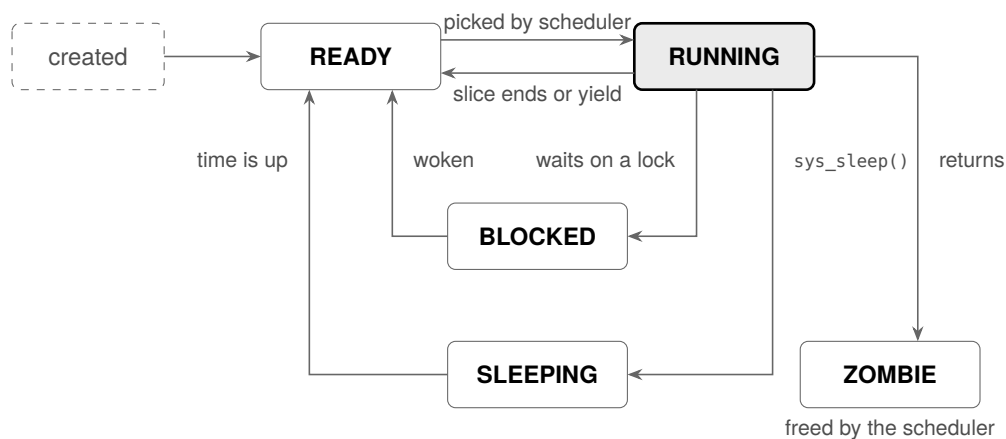
Figure 4.1: Thread states
