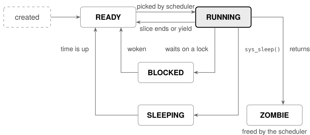
Figure 4.1: Thread states
