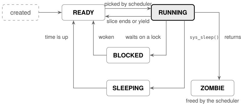
Figure 4.1: Thread states
