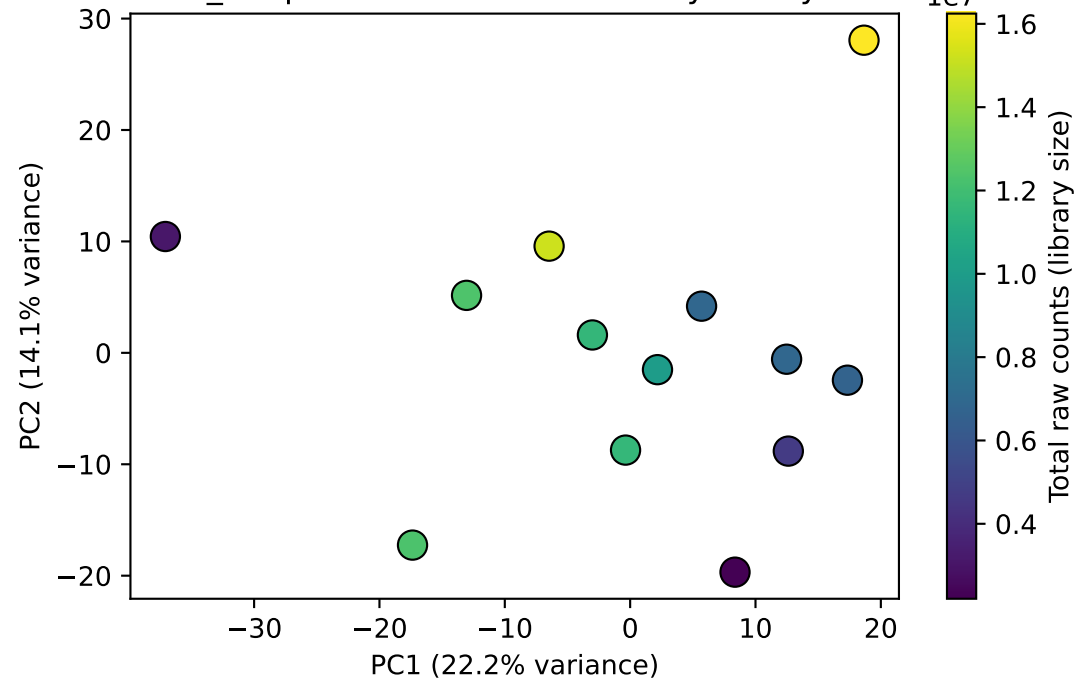
WAT_IPC pseudobulks — colored by library size
