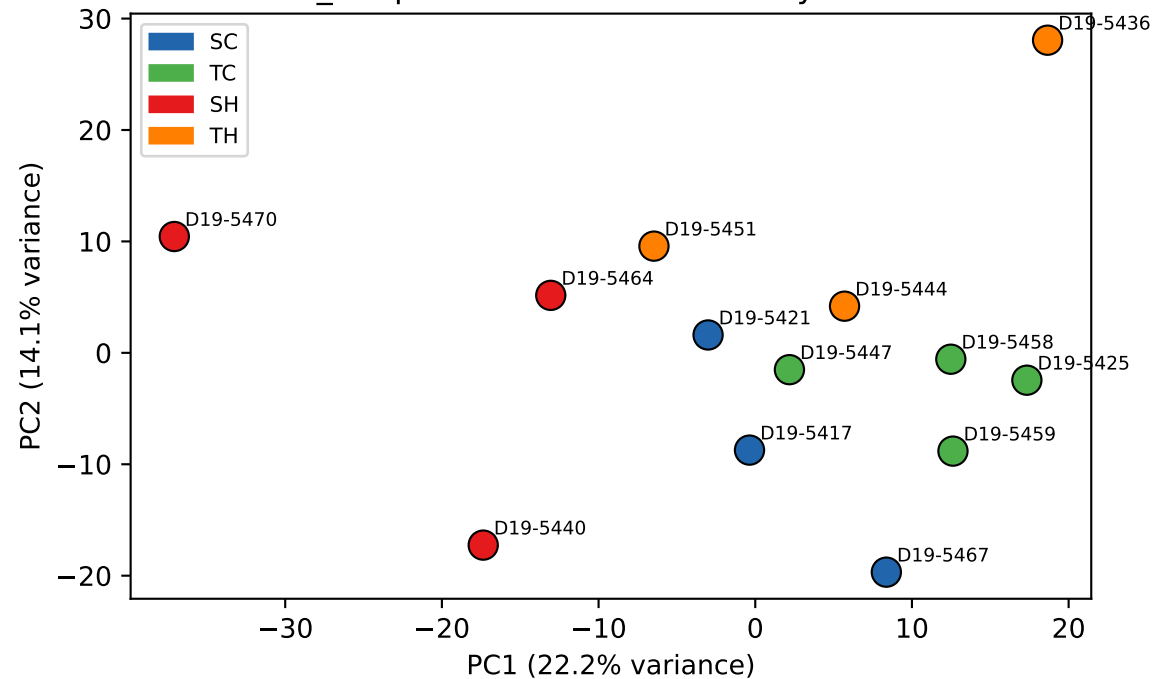
WAT_IPC pseudobulks — colored by condition
