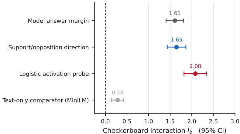
(a) Llama-3.1-8B-Instruct, layer 19
