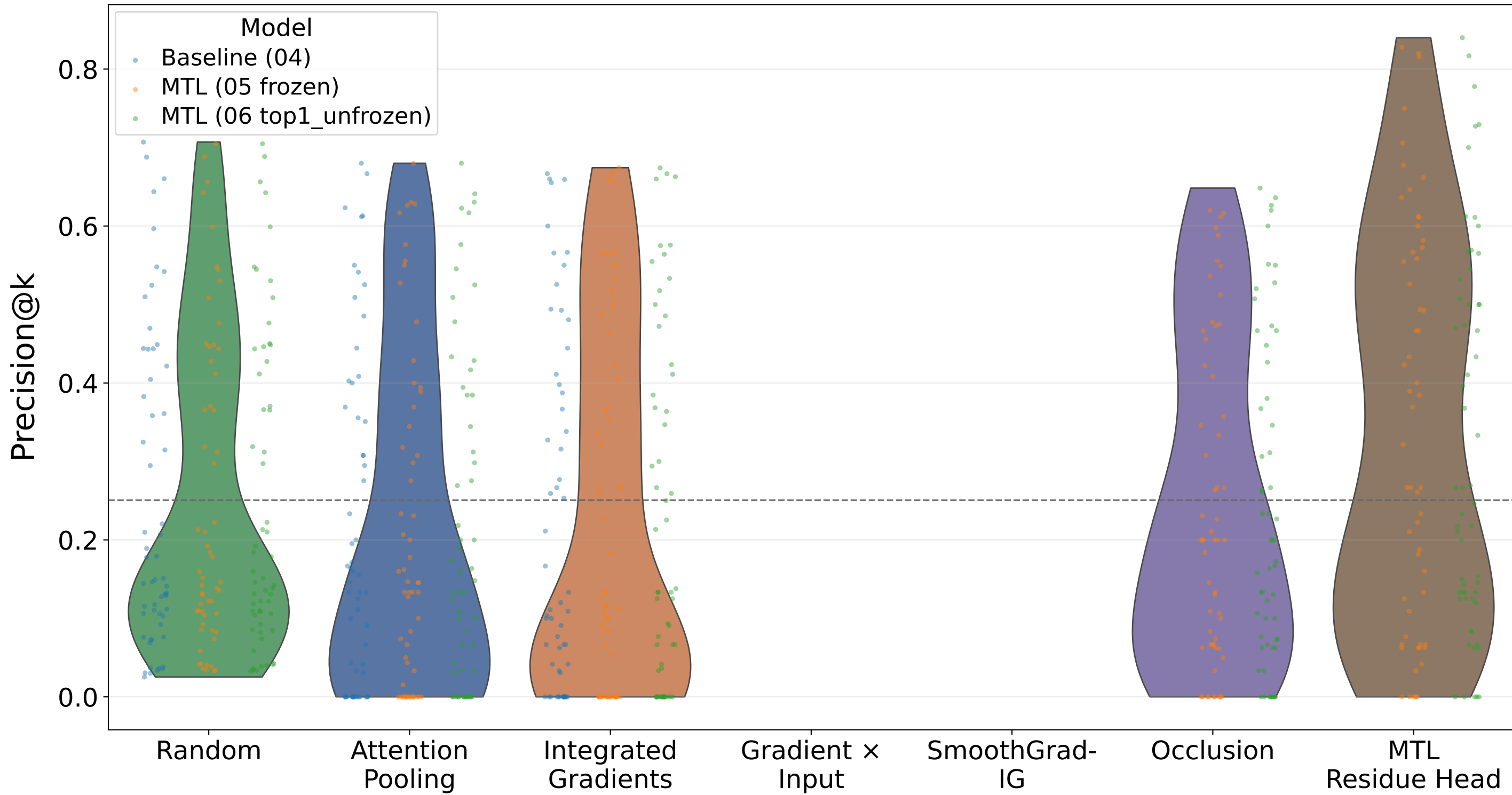
All Residue-Level Signals vs. IEDB Epitopes: Precision@k
