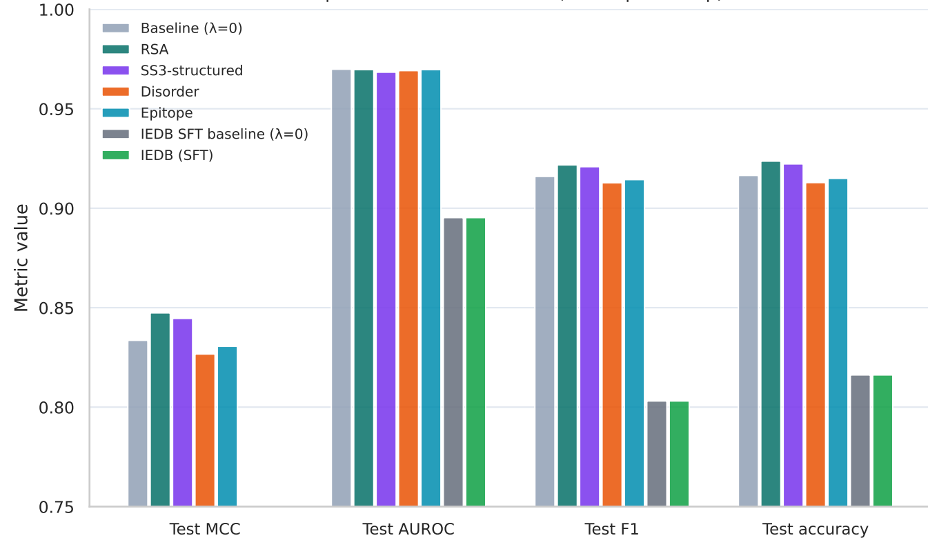
Sequence-level classification (best \lambda per sweep)
