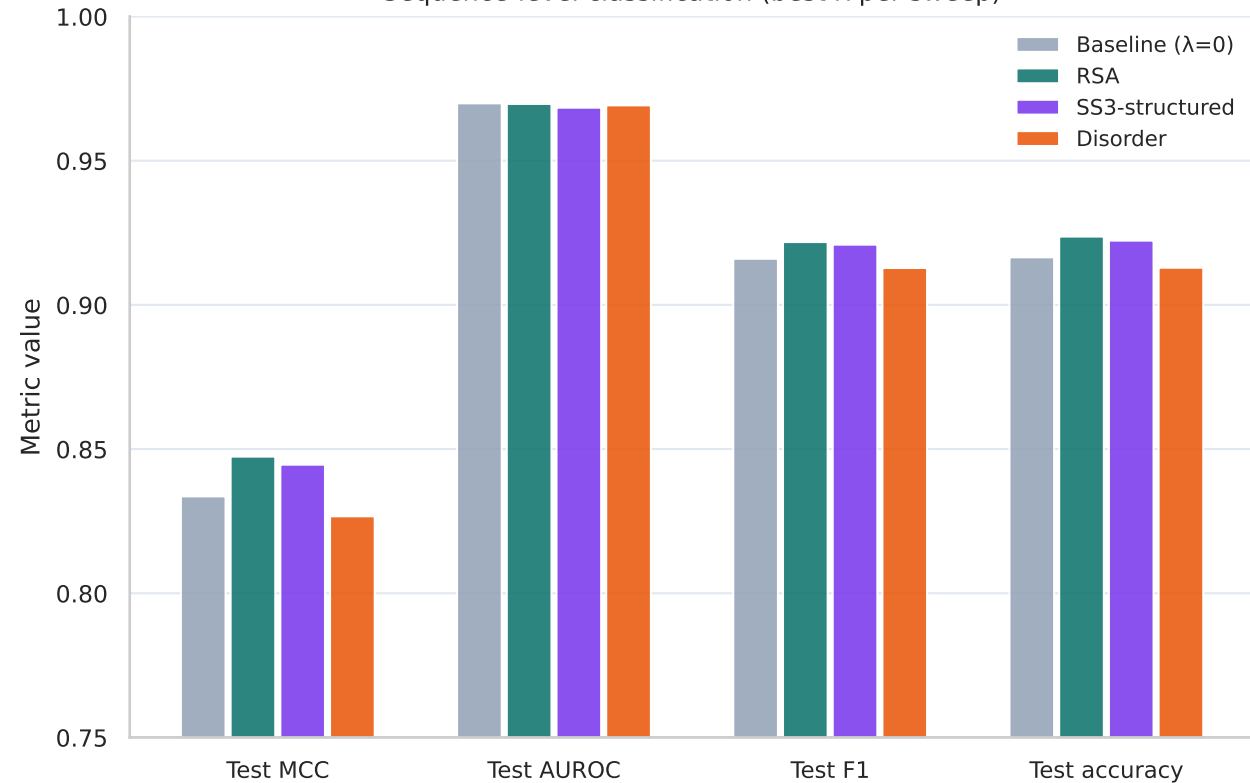
Sequence-level classification (best \lambda per sweep)
