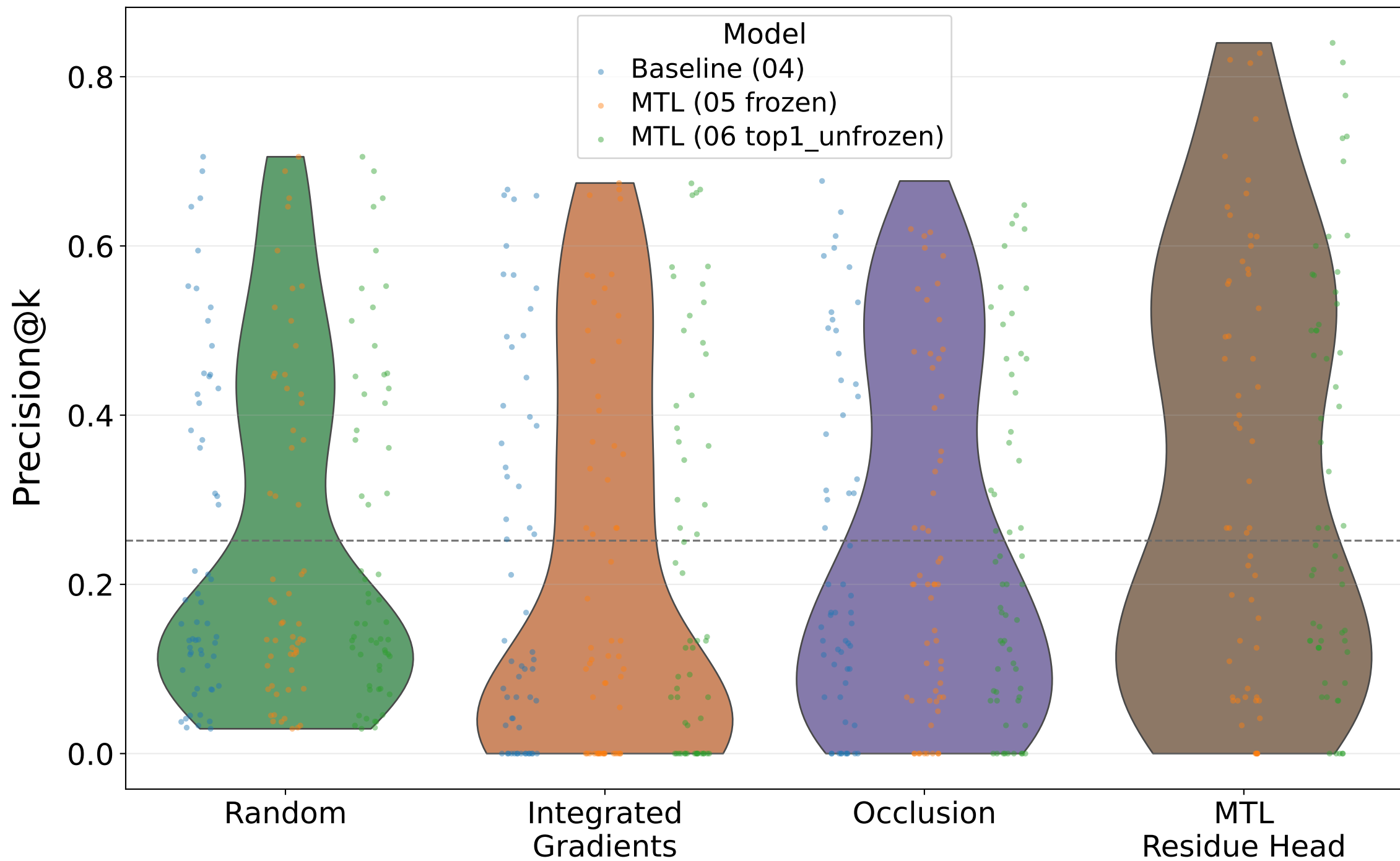
Residue-Level Localization vs. IEDB Epitopes: Precision@k
