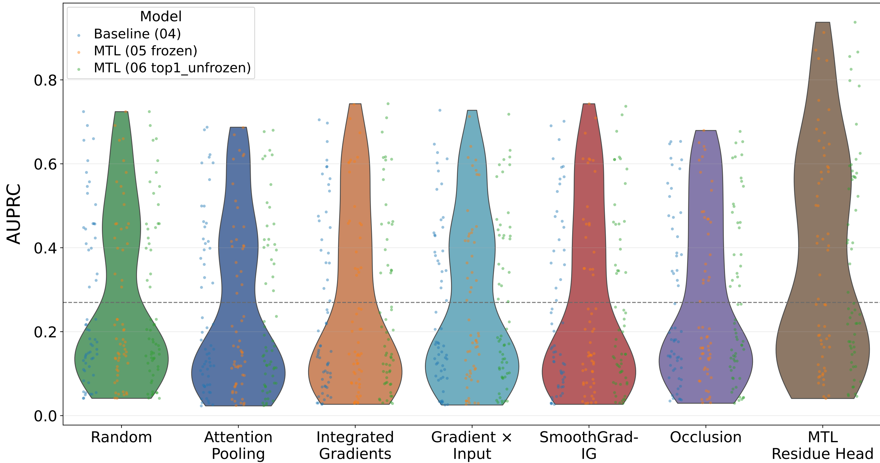
All Residue-Level Signals vs. IEDB Epitopes: AUPRC
