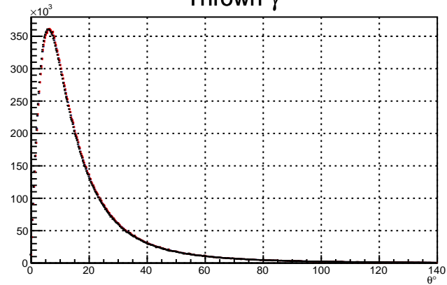
Thrown \gamma
