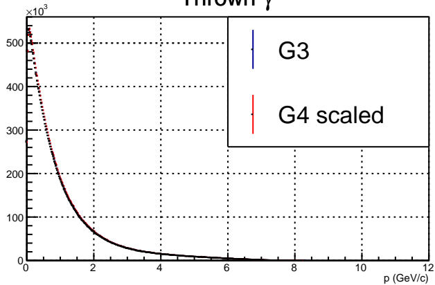
Thrown \gamma
