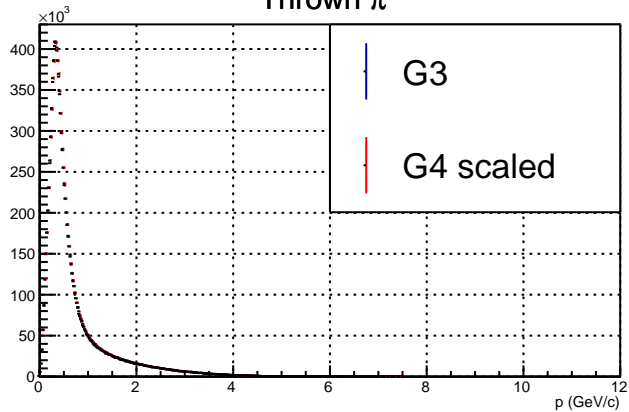
Thrown \pi^+
