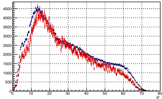
\rho, \gamma\rho \rightarrow \pi^+\pi^-\eta\rho
