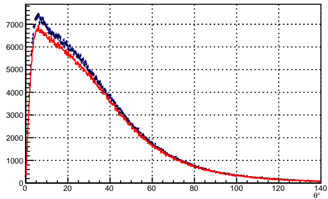
Thrown \pi^+
