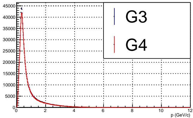
Thrown \pi^+
