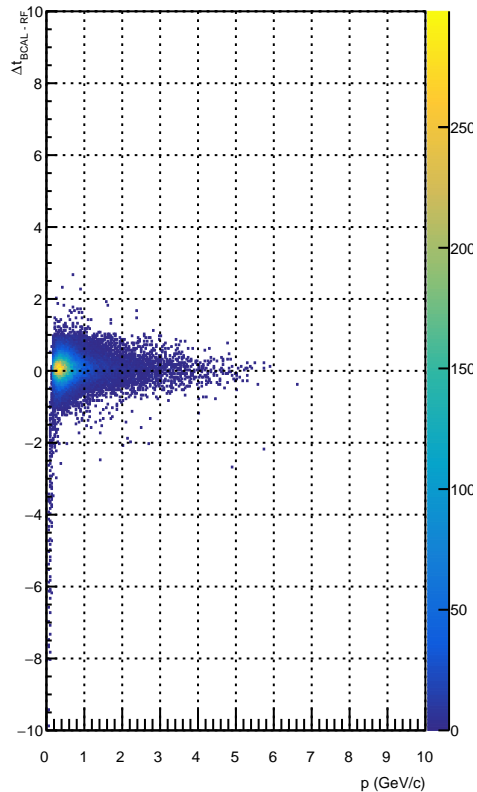
\pi^+ Candidates
