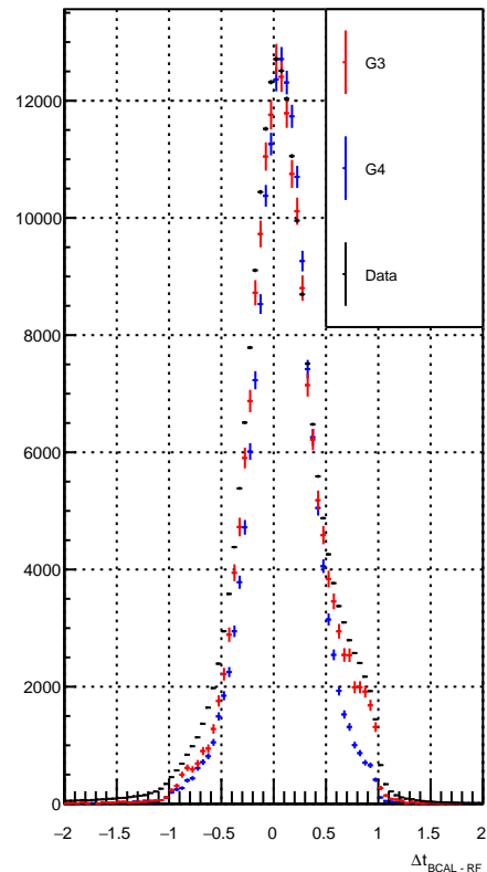
\pi^+ Candidates
