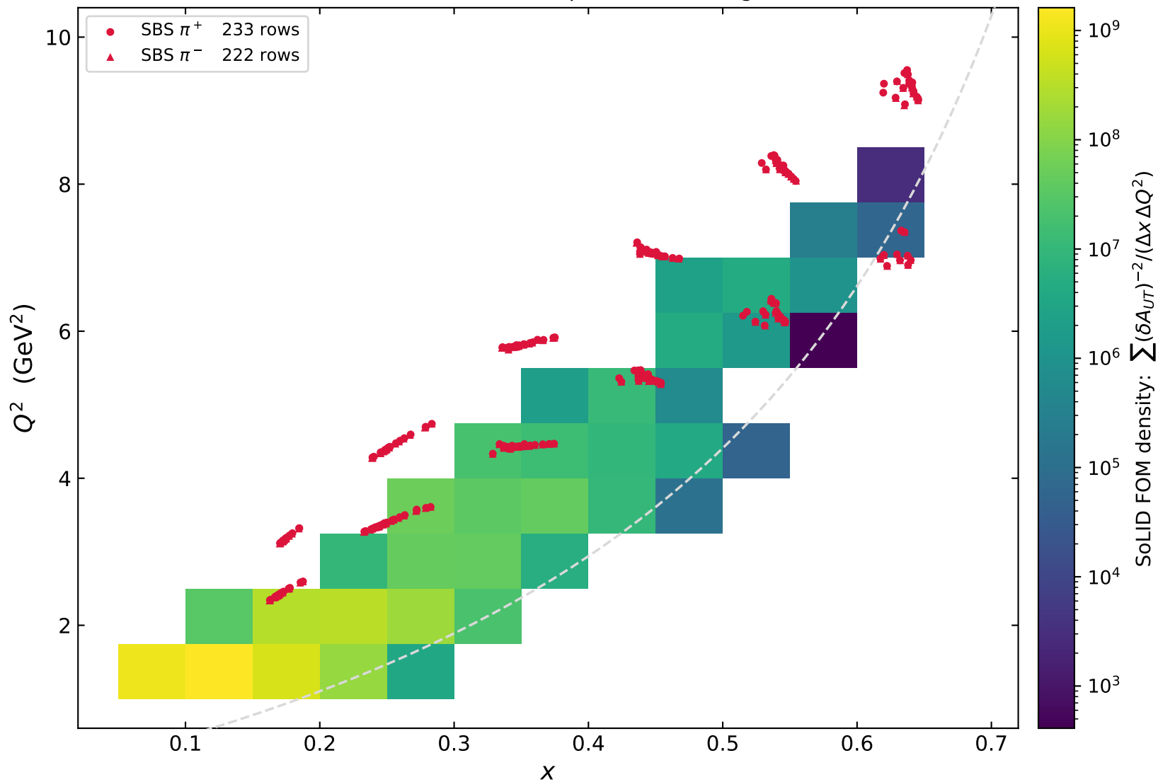
SoLID re-binned, SBS as points — nothing cut
