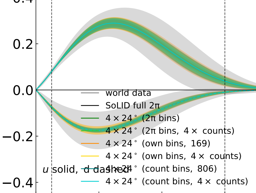
Collins 3He : azimuthal acceptance (stat. + syst.)
