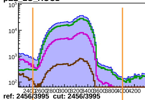
pEL_CLEAN_ROC1
