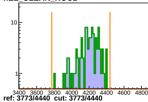
hEL_CLEAN_ROC1
