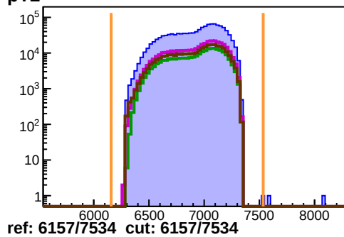
pT2
