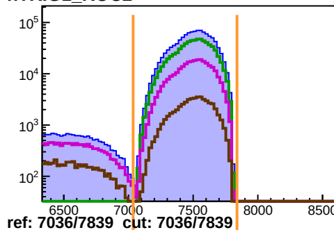
hTRIG4_ROC2
