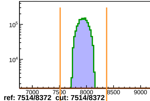
hTRIG4_ROC2
