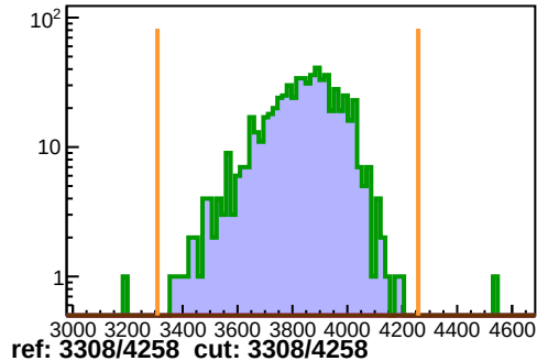
hT2
