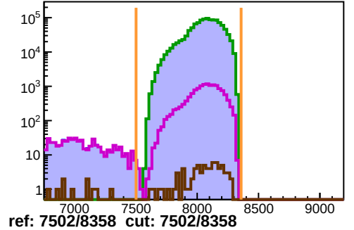
hTRIG4_ROC2
