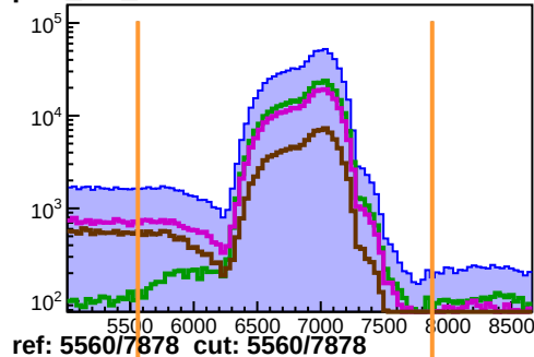
pEL_CLEAN_ROC2
