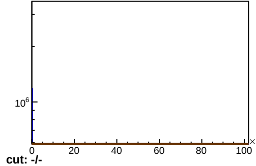
pSTOF_ROC2
