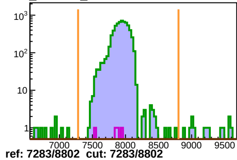
hEL_CLEAN_ROC2
