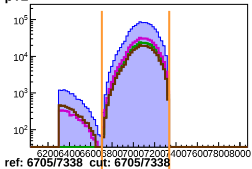
pT2
