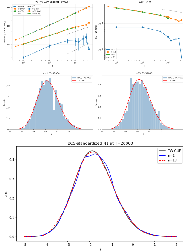
Figure 2: The Tracy–Widom regime. Left: \text{Cov}(N_1, N_2) \sim T^{1/2} , the uncorrelatedness of Conjecture 8.5. Middle: the marginal current against the GUE Tracy–Widom law F_2 at T = 3.3 \times 10^4 . Right: n -independence — the standardised marginals at n = 2 and n = 13 collapse onto F_2 .
