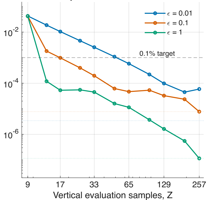
Exponential stratification
