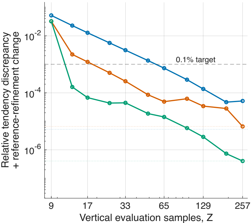
Constant stratification
