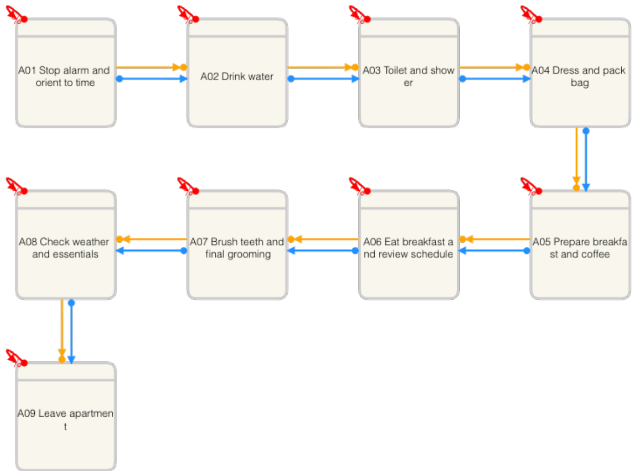
Figur 1: Interview-based DCR graph for the morning routine (A01-A09)
