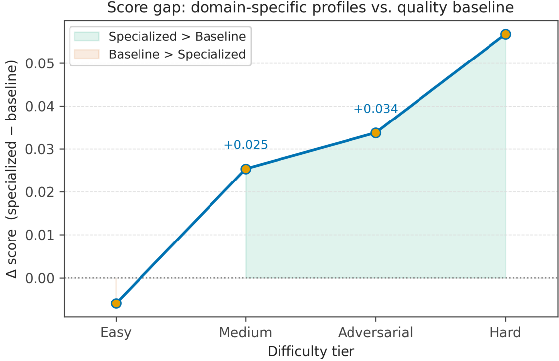
Figure 7: Score gap between domain-specific governance profiles and the quality baseline, by difficulty tier ( \Delta = \text{specialised} - \text{baseline} ). The monotonically increasing gap confirms that profile specialisation matters most on hard and adversarial content.
