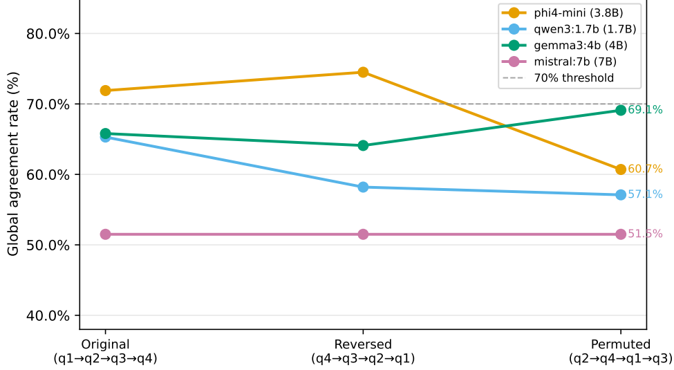
Figure 4: Global agreement rate per judge across three question orderings (original q1 \rightarrow q2 \rightarrow q3 \rightarrow q4 , reversed q4 \rightarrow q3 \rightarrow q2 \rightarrow q1 , permuted q2 \rightarrow q4 \rightarrow q1 \rightarrow q3 ) on the 49-case ground truth corpus. Each point is the weighted average across five criteria. The dashed line marks the 70% reliability threshold used for judge classification. mistral:7b is flat across all three orderings (51.5%), indicating structural miscalibration rather than positional sensitivity. phi4-mini is stable between original and reversed (+2.6 pp) but collapses on permuted (−11.2 pp), revealing conditional robustness. gemma3:4b improves on permuted (+3.3 pp vs. original), consistent with its internal reasoning structure.
