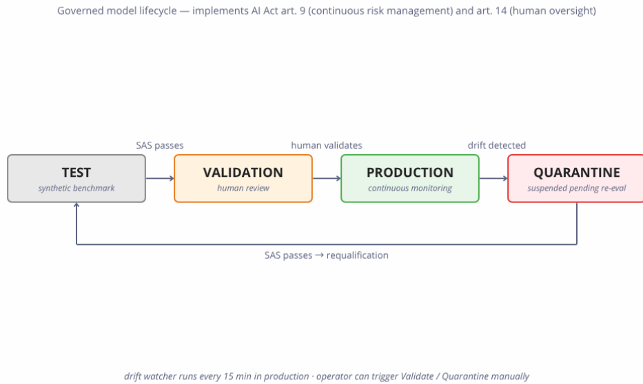
Figure 3: Model lifecycle qualification cycle. A model advances from test to production only after explicit human validation against governance thresholds; score degradation below a configurable threshold triggers automatic quarantine. The cycle implements AI Act art. 9 (continuous risk management) and art. 14 (human oversight gate).
