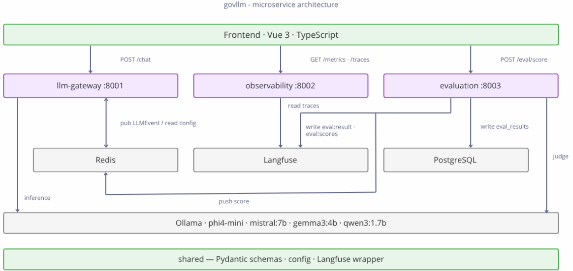
Figure 1: Microservice architecture of govllm . Three independent FastAPI services share a common Pydantic schema library. The gateway publishes observability events to Redis; judge evaluation is triggered by the frontend via a direct call to POST /eval/score on the evaluation service.
