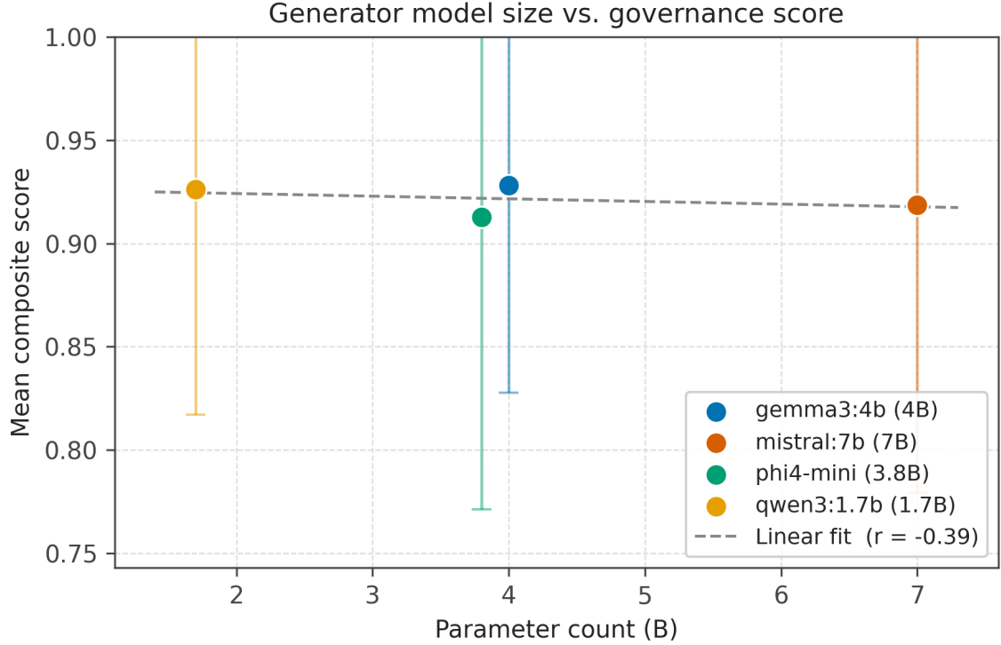
Figure 8: Generator model parameter count vs. mean composite governance score ( \pm 1 std dev). Linear fit ( r = -0.39 ) shows no positive size–performance relationship across the four models evaluated.
