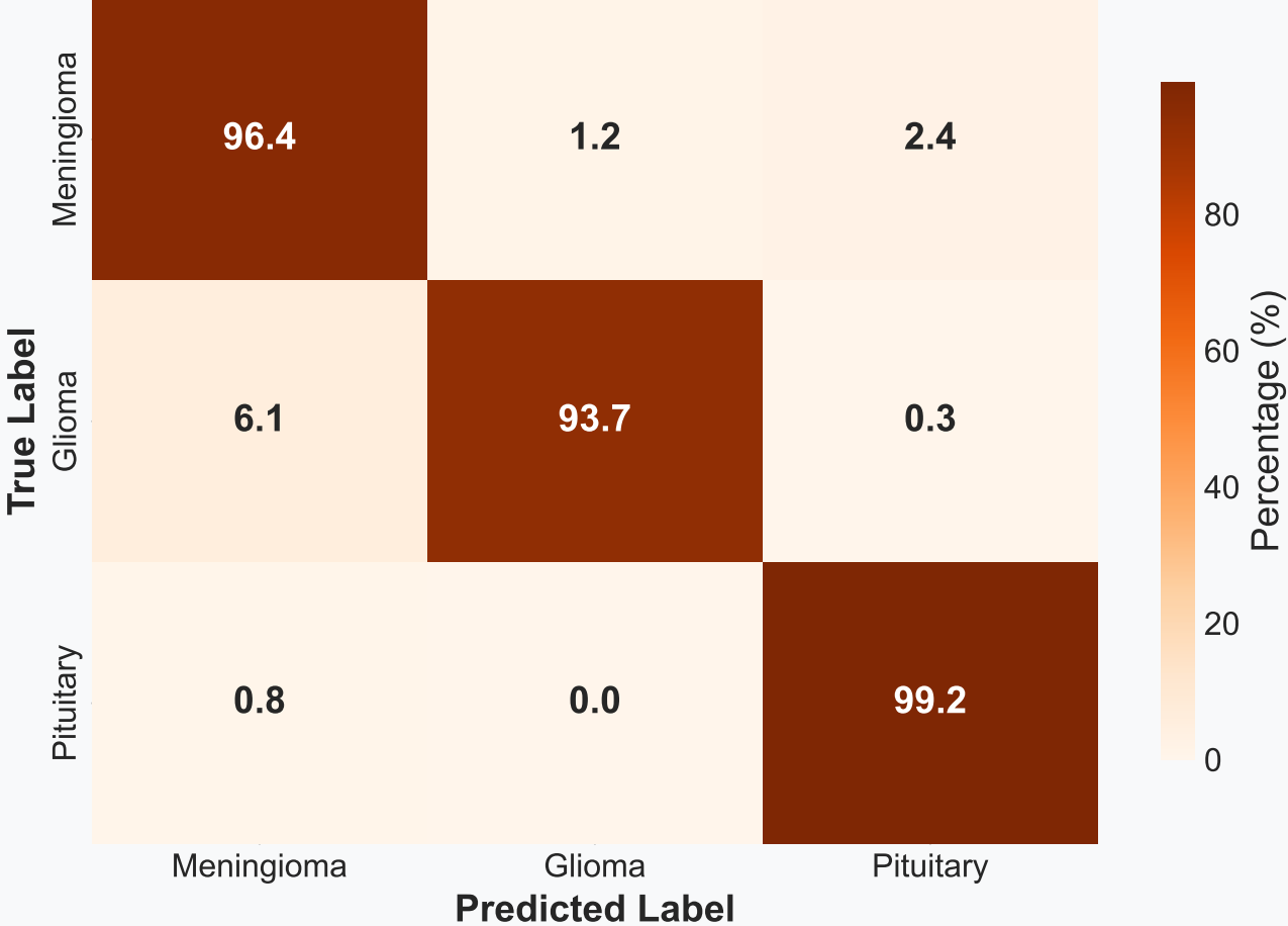
Stage 2: Confusion Matrix - Percentages
