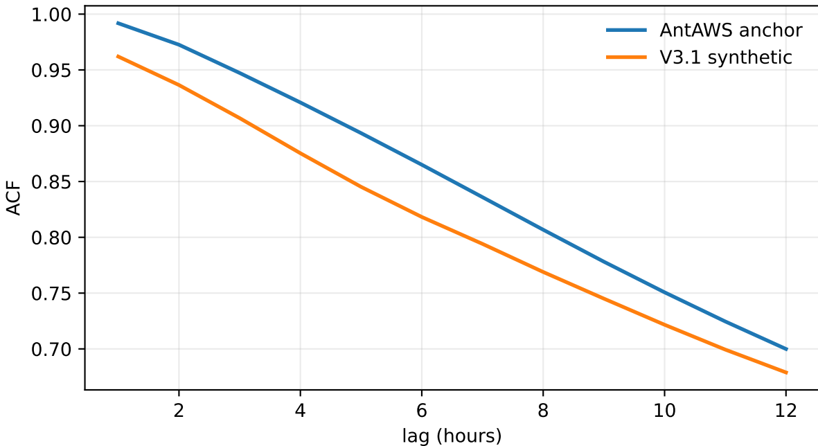
Wind-speed autocorrelation
