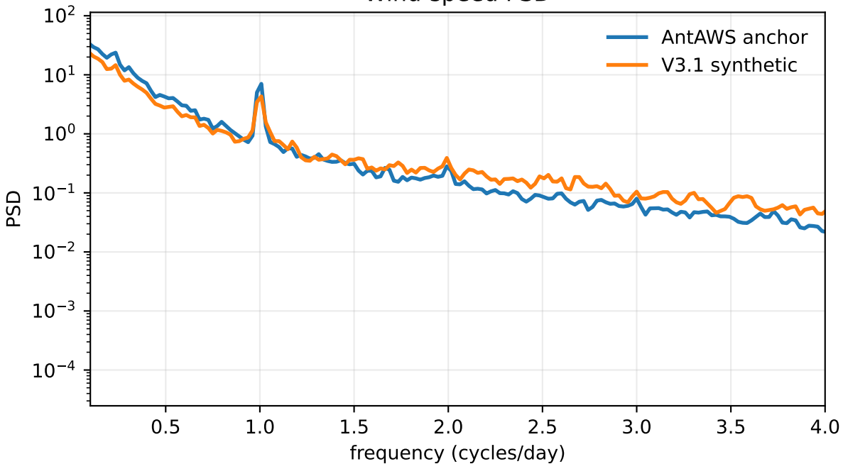
Wind-speed PSD
