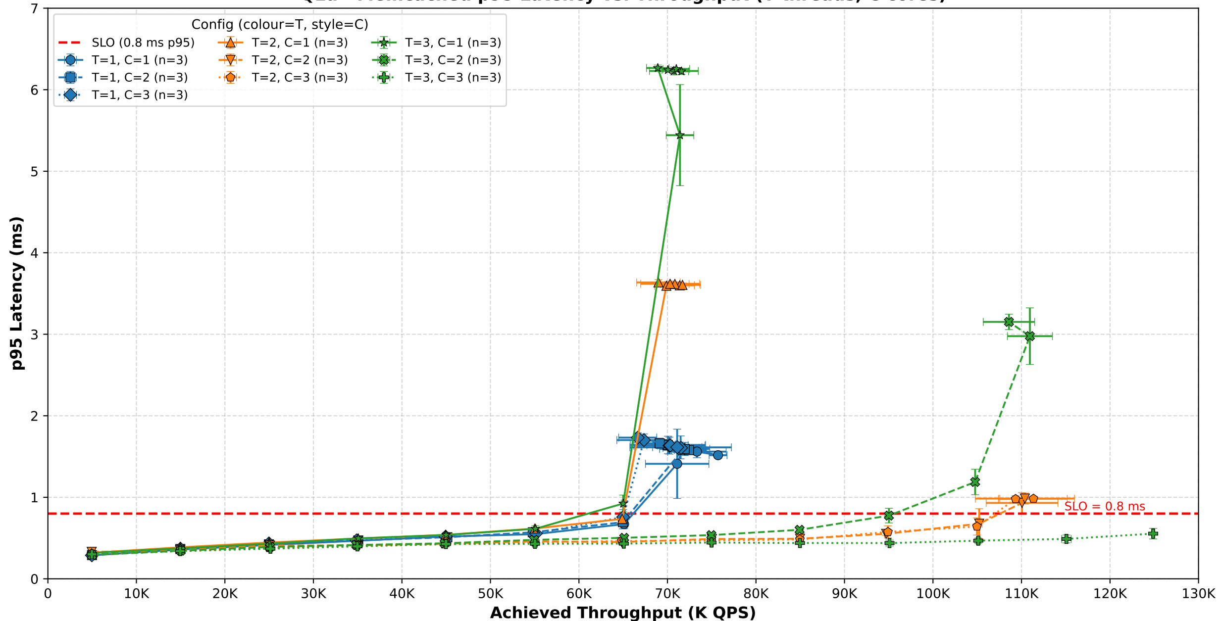
Q1a - Memcached p95 Latency vs. Throughput (T threads, C cores)
