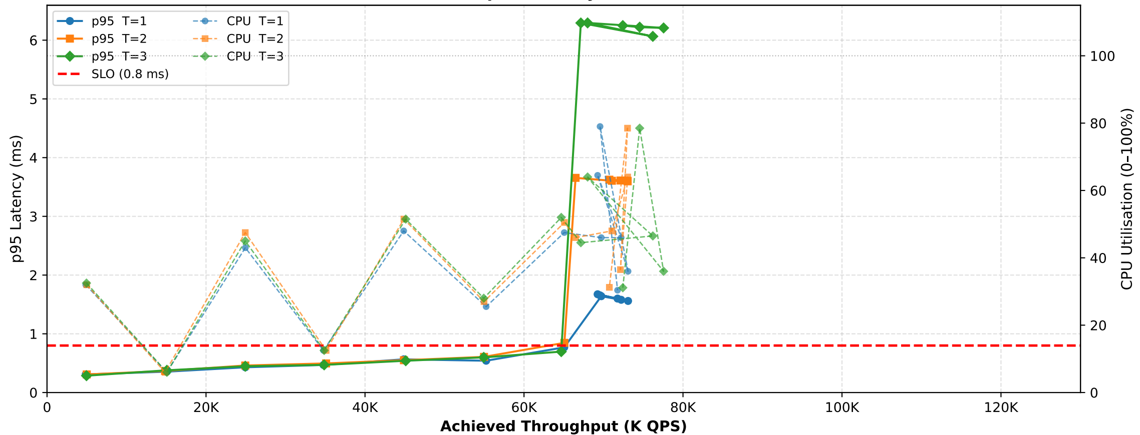
Q1d — C=1 core(s): p95 Latency and CPU util for T=1,2,3
