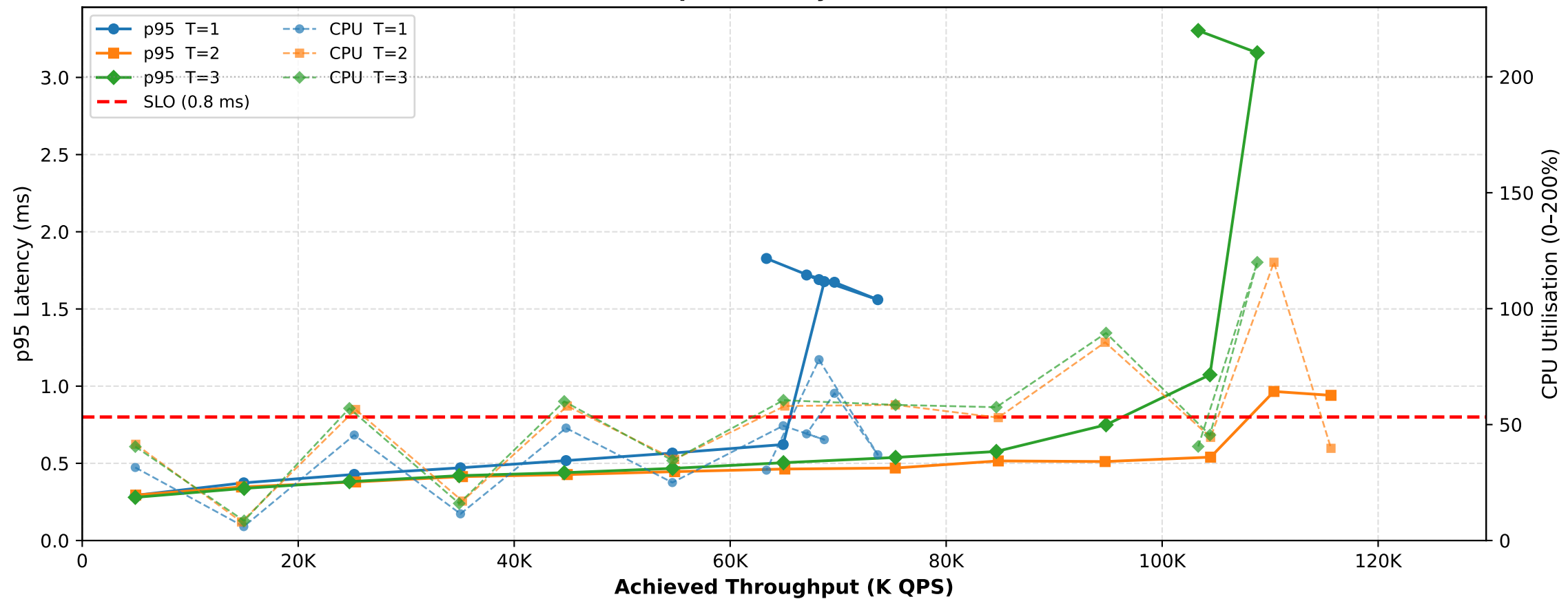
Q1d — C=2 core(s): p95 Latency and CPU util for T=1,2,3
