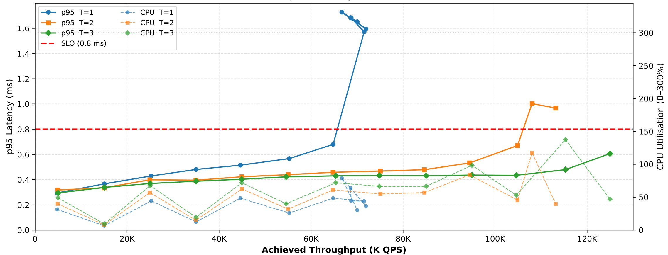
Q1d — C=3 core(s): p95 Latency and CPU util for T=1,2,3
